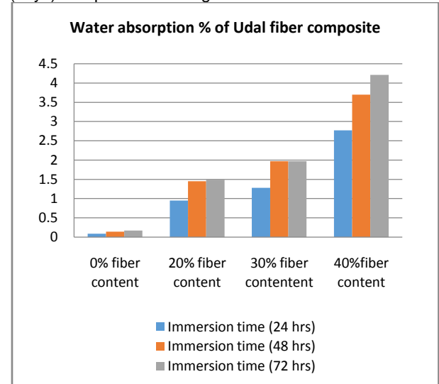
Fig.3: Water absorption %
